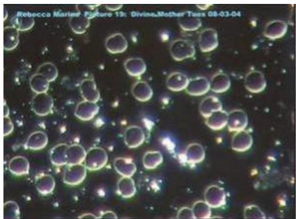
Figure 9. Blood molecules
