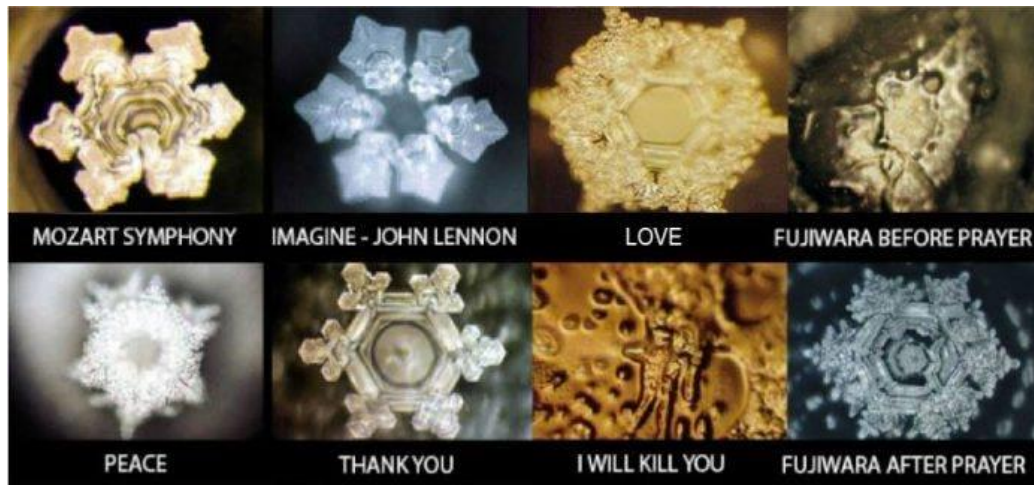
Figure 4. Emoto's results 8
