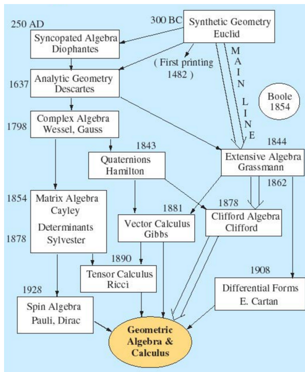
Figure 1: Geometric Algebra timeline [37]
