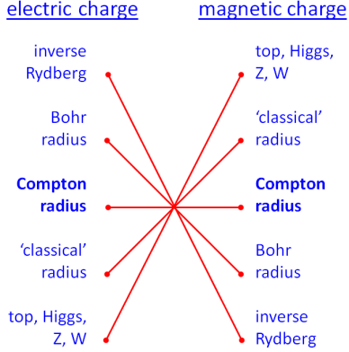
Figure 3: Topological inversion
