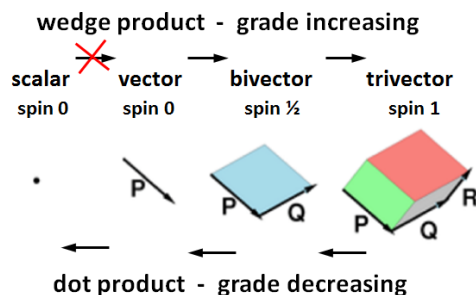
Figure 2: Pauli algebra of 3D space
