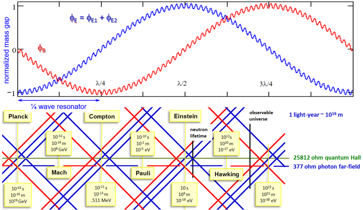
Figure 11: Hawking photon attenuation by impedance mismatch reflections [27, 64–66]
