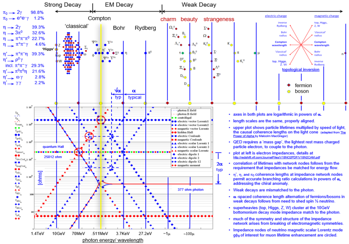
Figure 9: Correlation of lifetimes with \alpha -spaced network nodes [27, 64–66]
