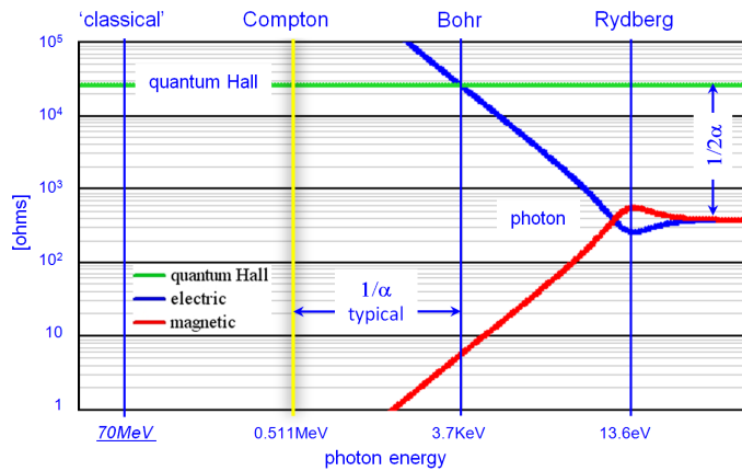
Figure 6: H atom impedance match [25]
