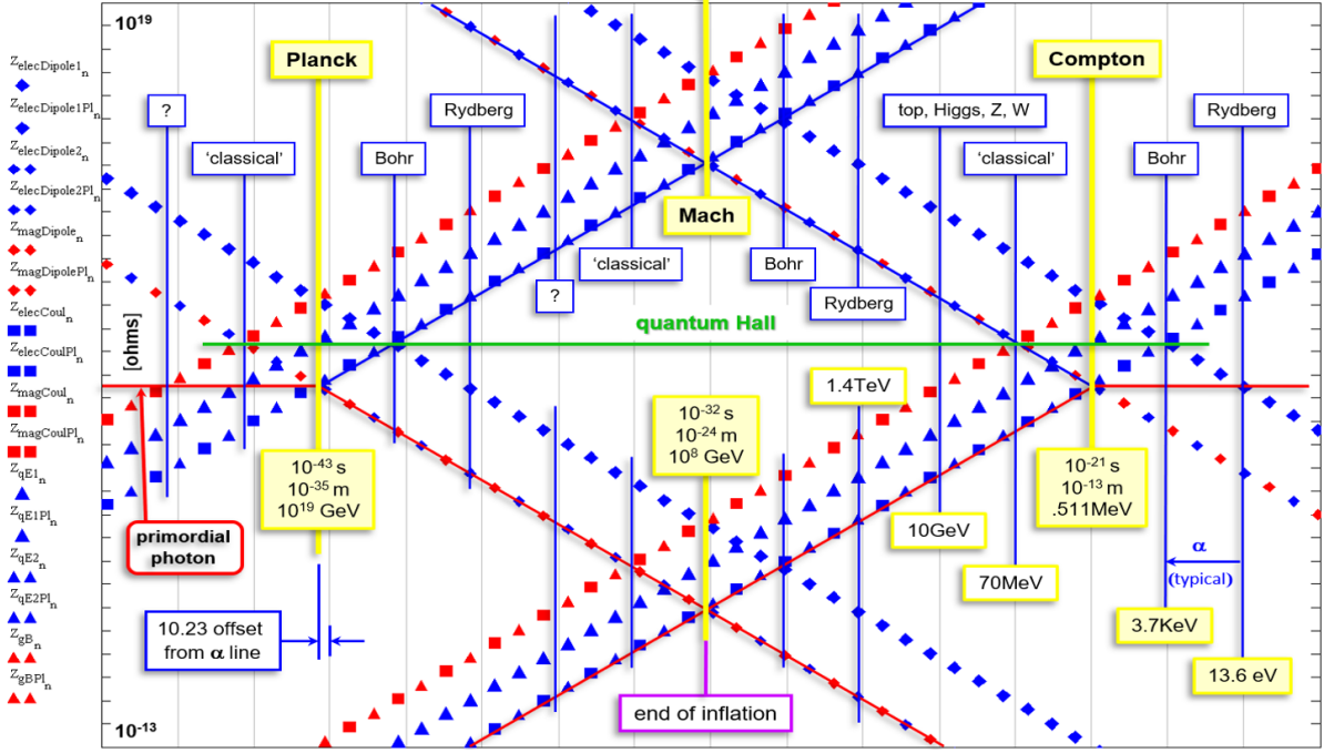
Figure 10: Interaction impedance networks defined at Compton and Planck lengths, showing a .511 Mev photon entering from right and ‘primordial photon’ from left. [96–98]
