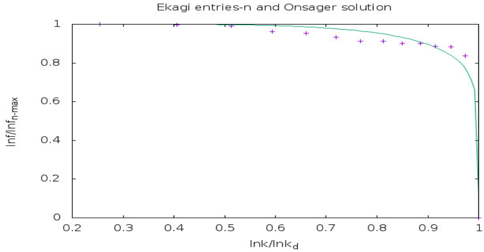
FIG. 4. The vertical axis is \frac{\ln f}{\ln f_{next-max}} and the horizontal axis is \frac{\ln k}{\ln k_{lim}} . The + points represent the entries of the Ekagi language. The reference curve is the Onsager solution.
