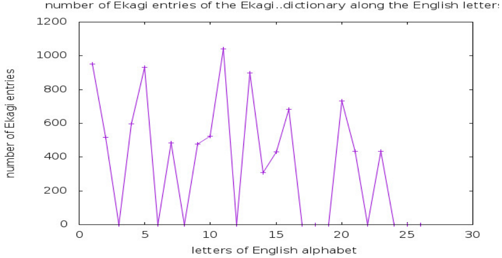
FIG. 2. The vertical axis is number of entries of the Ekagi language and the the horizontal axis is the respective letters of the Ekagi alphabet. Letters are represented by the sequence number in the English alphabet beginning with A.
