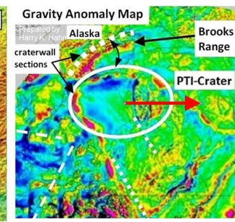
Gravity Anomaly Map
