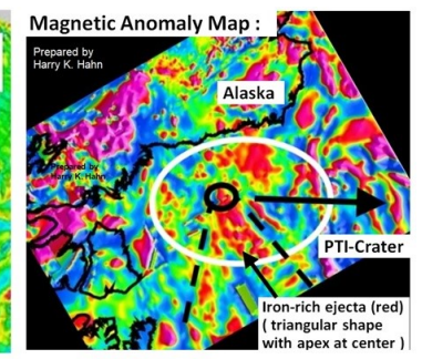
Magnetic Anomaly Map : Iron-rich ejecta (red) (triangular shape with apex at center)
