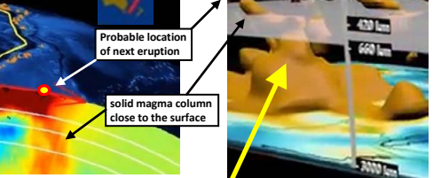
3D-Model No. 1 of Pacific LLSVP → see : 3D-Animation 1 3D-Model No. 2 of Pacific LLSVP → see : 3D-Animation 2
