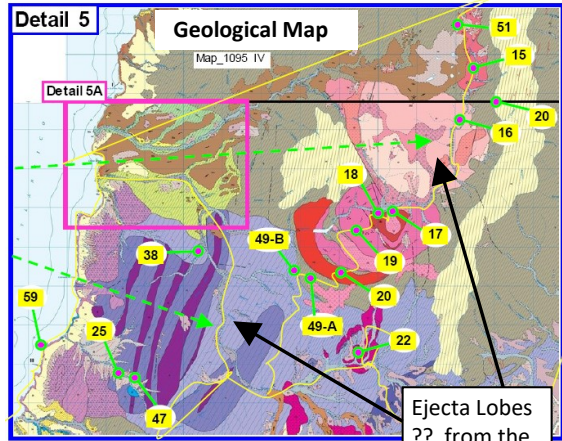
fragment of old Mesozoic Oceanic Crust
