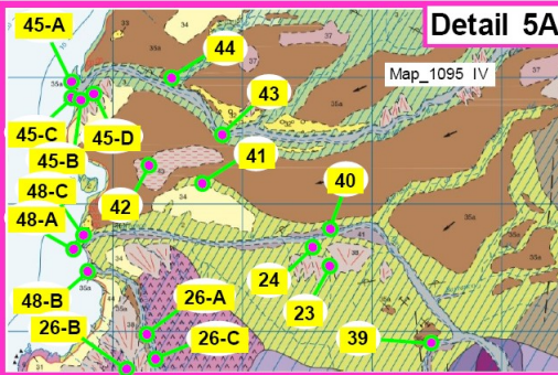
fragment of old Mesozoic Oceanic Crust
