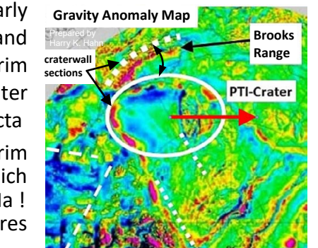
Note similarity of bow-shaped structure ! → structure was caused by the motion of the impactor along the surface
