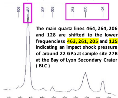
The Raman Spectra of quartz grains from sample site 27B at the BLC shows a clear shift of main quartz peaks to lower frequencies
