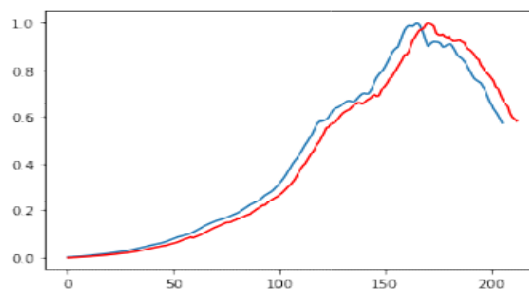
Figure 5(b): LSTM training data
