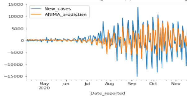
Figure 4: ARIMA prediction
