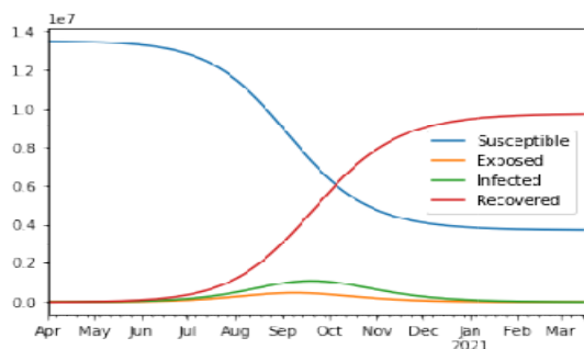
Figure 3(a): SEIR model for Indian cases
