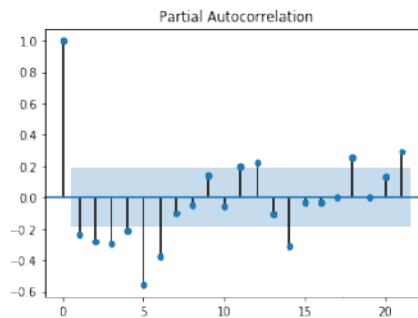
Figure 2(d): PACF graph after differencing(2)
