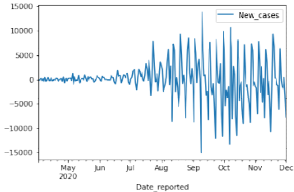
Figure 2(a): 1-Differenced data with p-value:0.4
