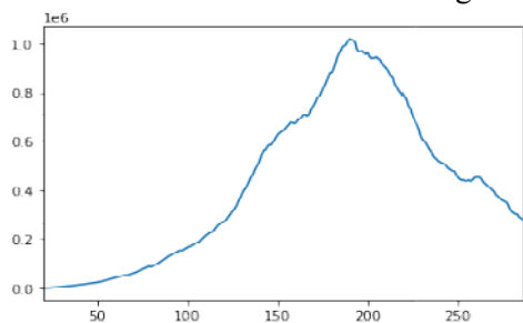
Figure 5(a): Daily Active cases(Total)
