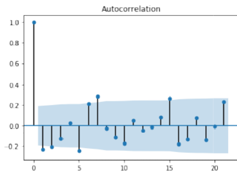
Figure 2(c): ACF graph after differencing(2)
