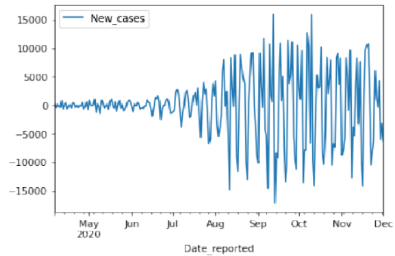
Figure 2(b): 2-Differenced data with p-value: 0.002
