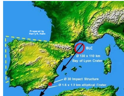
This map shows the three most interesting PT-Secondary Craters for further research in Europe, according to my analysis.
