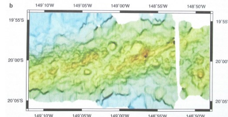
Fig. 1.12. a Bathymetry of a segment of the Vā'a Tau Pitā Ridges near Tahiti (Clouard et al. 2003). These volcanic ridges are clearly constructed by the superposition of many small, flat-topped volcanic cones. The Simrad EM12D, Hydrosweep DS and SeaBeam multibeam bathymetry is shown using a 100 m grid interval and shading by slope magnitude. b Detail of volcanic morphology of ridges in region shown by box in a
