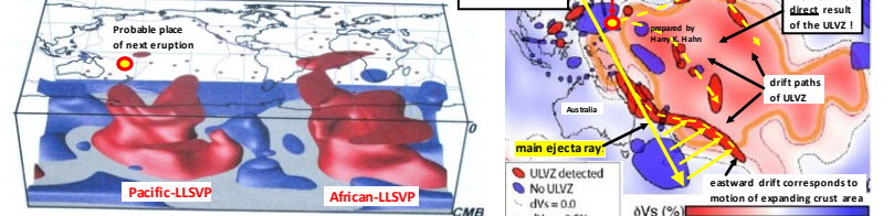
A 3-D view of the Pacific- & African LLSVP and the probable location of the next eruption
