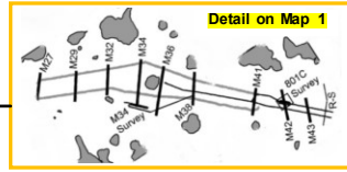
Chron Numbers of Magnetic Lineations in North-Pacific
