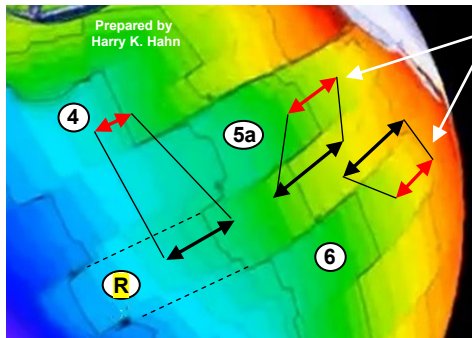
The marked areas on the stripes 4, 5a & 6 (red arrows) indicate compressed areas, if compared with reference stripe " R " which probably was not effected by an eruption
