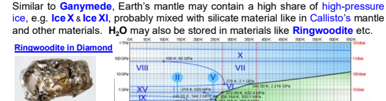
An alternative model for Earth's mantle is required !! Earth's mantle in all probability contains much more volatiles , especially H 2 O, than currently believed ! Similar to Ganymede , Earth's mantle may contain a high share of high-pressure ice , e.g. Ice X & Ice XI , probably mixed with silicate material like in Callisto's mantle and other materials. H 2 O may also be stored in materials like Ringwoodite etc.
