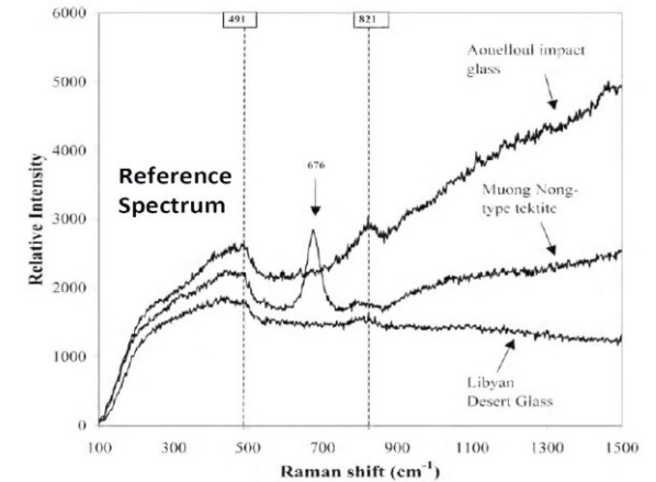
Fig. 8. Raman spectra of Aouelloul impact glass (a), Muong Nong-type tektite (b), and Libyan desert glass (c) generally exhibit two broad bands at 491 and 821 cm -1 and relatively high background fluorescence, which indicate a high degree of amorphization. These broad bands might be due to diaplectic glass. The numbers denote peak positions in cm -1 .
