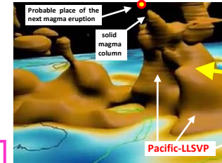
3D-view of Pacific-LLSVP with possible location of next eruption
