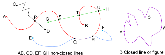
Figure 1 – A, B: endpoints of AB; C, D: endpoints of CD etc. AB, EF: locally collinear. AP, PS: adjacent at P. AP, PB: sides of P in AB. QR: common segment of AB y EF. S is between A y Q; between P and R etc.
