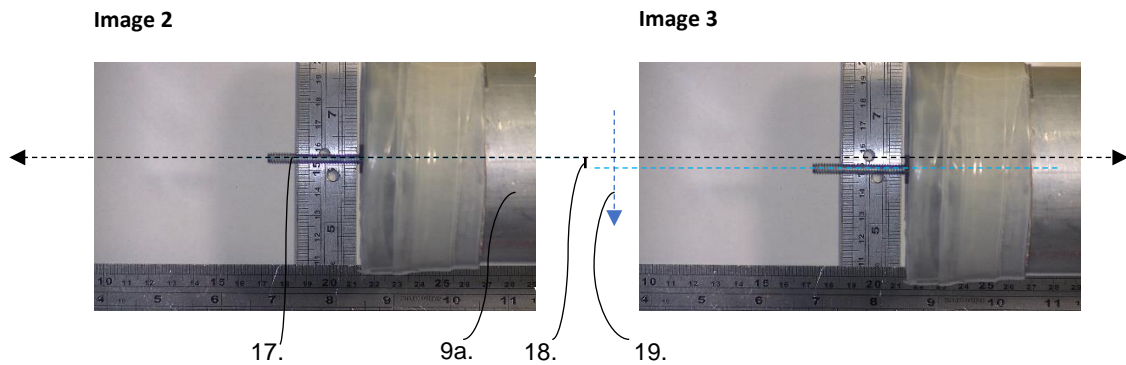
Images 2-3: spring-suspended resonance chamber (9.) showing a 5mm (18.) movement (19.) by the movement-marker (17.) from image 2 to image 3 (30s time-period from image 2 (0s) to image 3 (30s) during RF activation).
