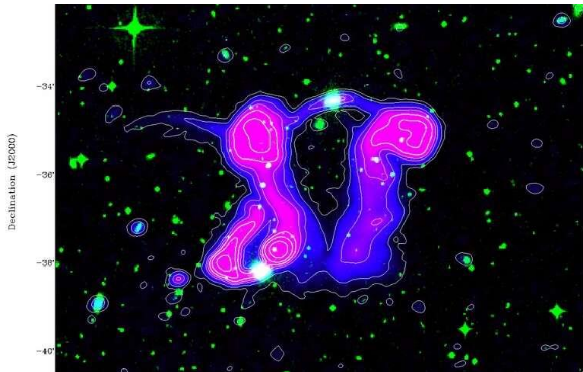
Two 'dancing ghosts' recently discovered using ASKAP, which might be a binary system of black holes about to merge. Credit: Baerbel Koribalski / CSIRO
