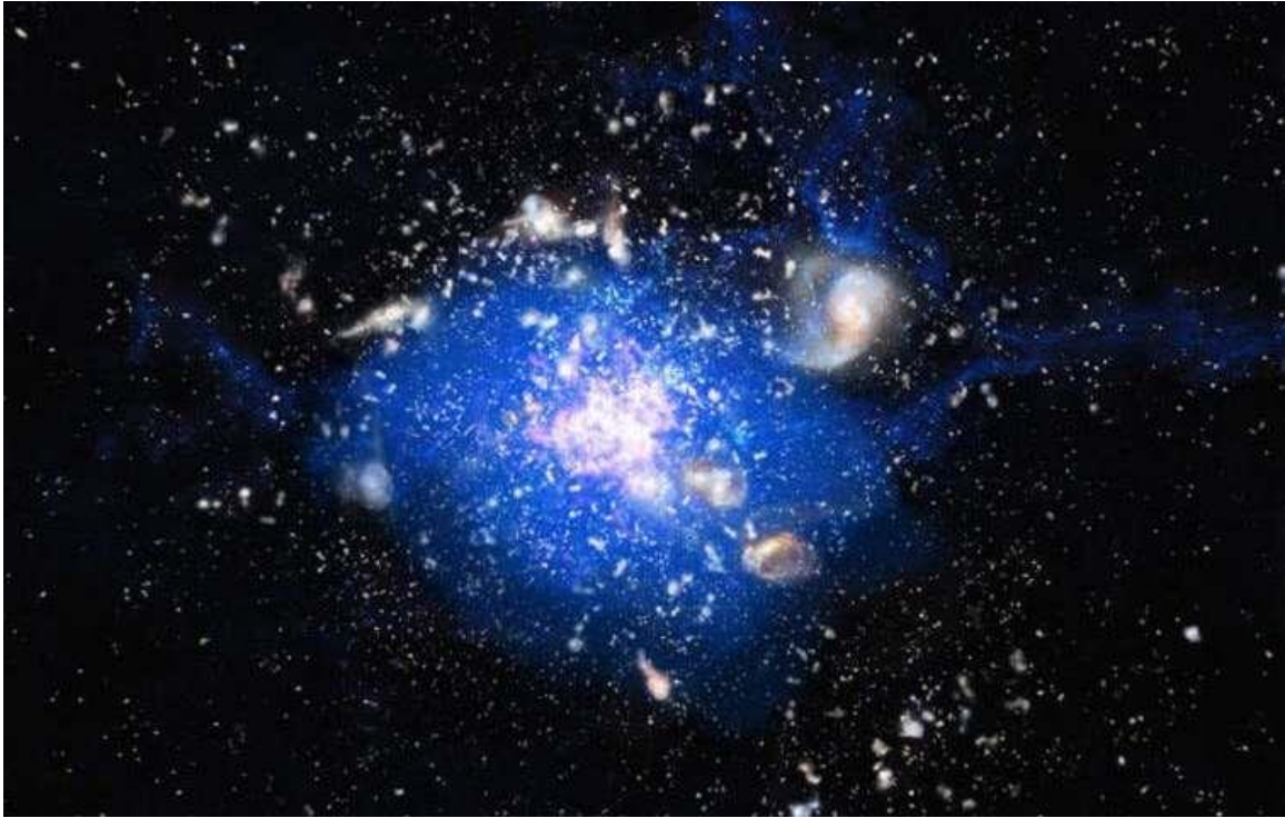
Carbon monoxide gas (shown in blue) in the Spiderweb cluster of galaxies, 10 billion light years away, observed with the ATCA by Bjorn Emonts and colleagues. Credit: M. Kornmesser / ESO.
