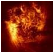
Hydrogen gas in the Large Magellanic Cloud, a companion galaxy to our own Milky Way, observed with the ATCA by Sungeun Kim and colleagues. Credit: CSIRO
