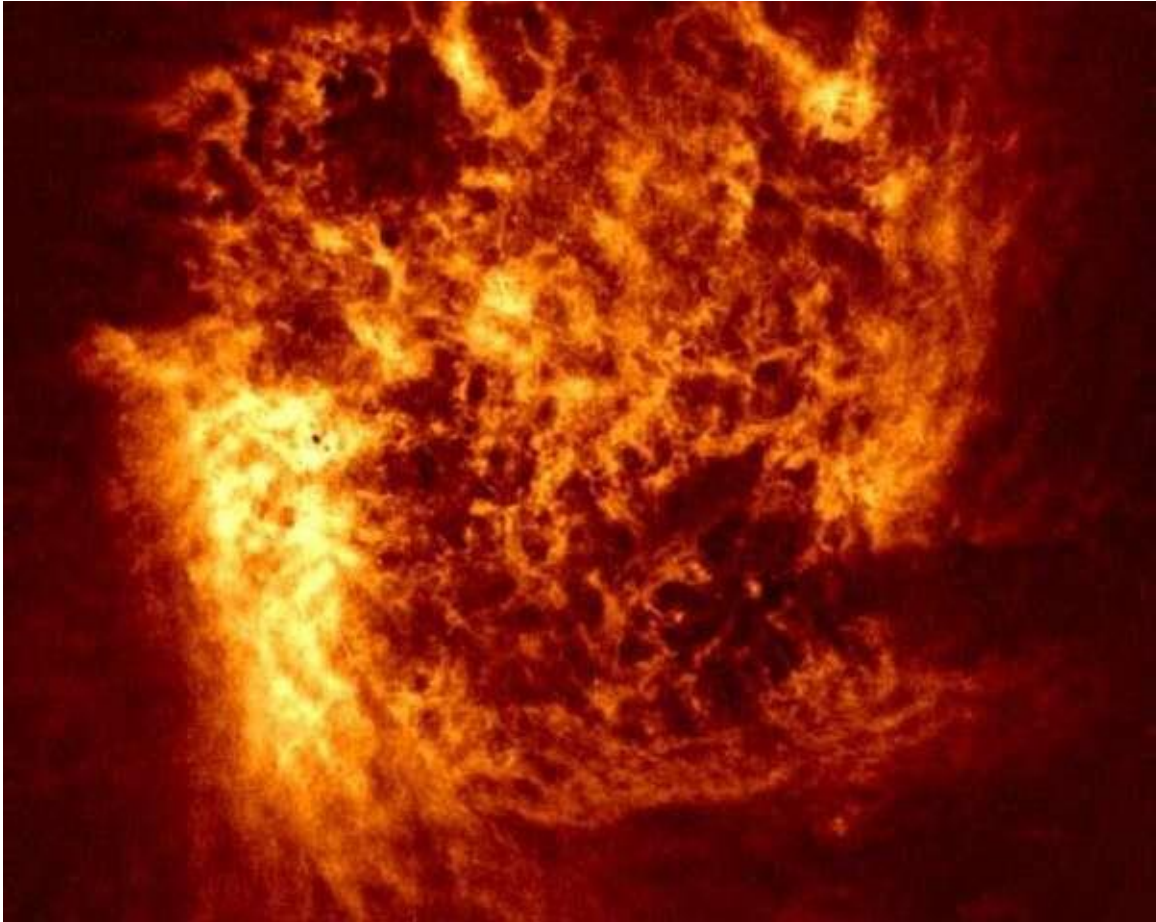
Hydrogen gas in the Large Magellanic Cloud, a companion galaxy to our own Milky Way, observed with the ATCA by Sungeun Kim and colleagues. Credit: CSIRO
