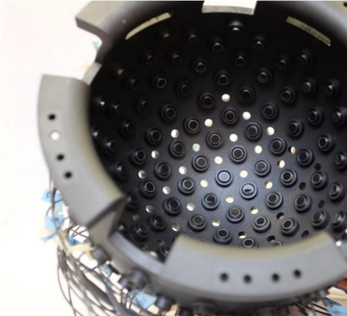
A prototype array with 120 ultrasound transducers. (Courtesy: L Guasch et al )
