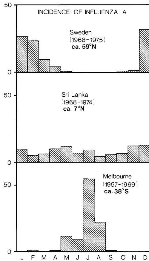
Figure. C Incidence of seasonal influenza A in 3 countries (Reproduced from Hoyle and Wickramasinghe: Proofs that Life is Cosmic , 1982) Figure copyright Chandra Wickramasinghe.
