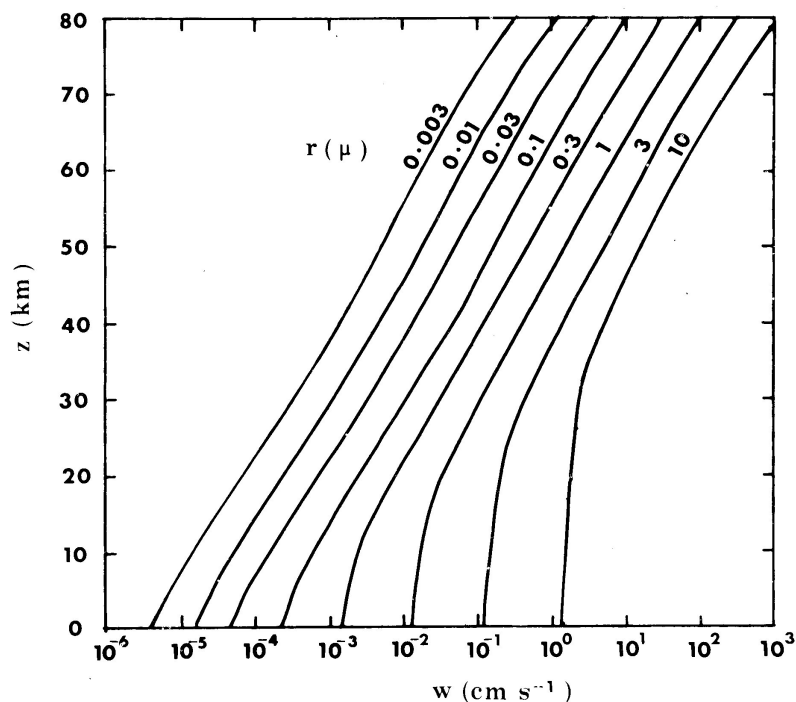
Figure .A . Falling speed of spherical dust particles as a function of height in the atmosphere (reproduced from Hoyle & Wickramasinghe, Proofs that Life is Cosmic , Mem. Inst.Fund.Studies, Sri Lanka, 1982) (copyright Chandra Wickramasinghe)
