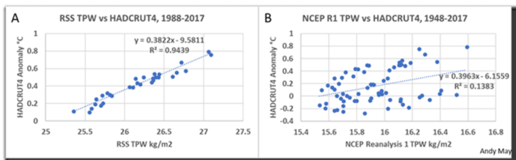
Figure 8 Correlation of specific humidity - Total Precipitation Water (TPW) for different data with global warming [8]. Here the author does not differentiate between specific humidity and atm. precipitation.
