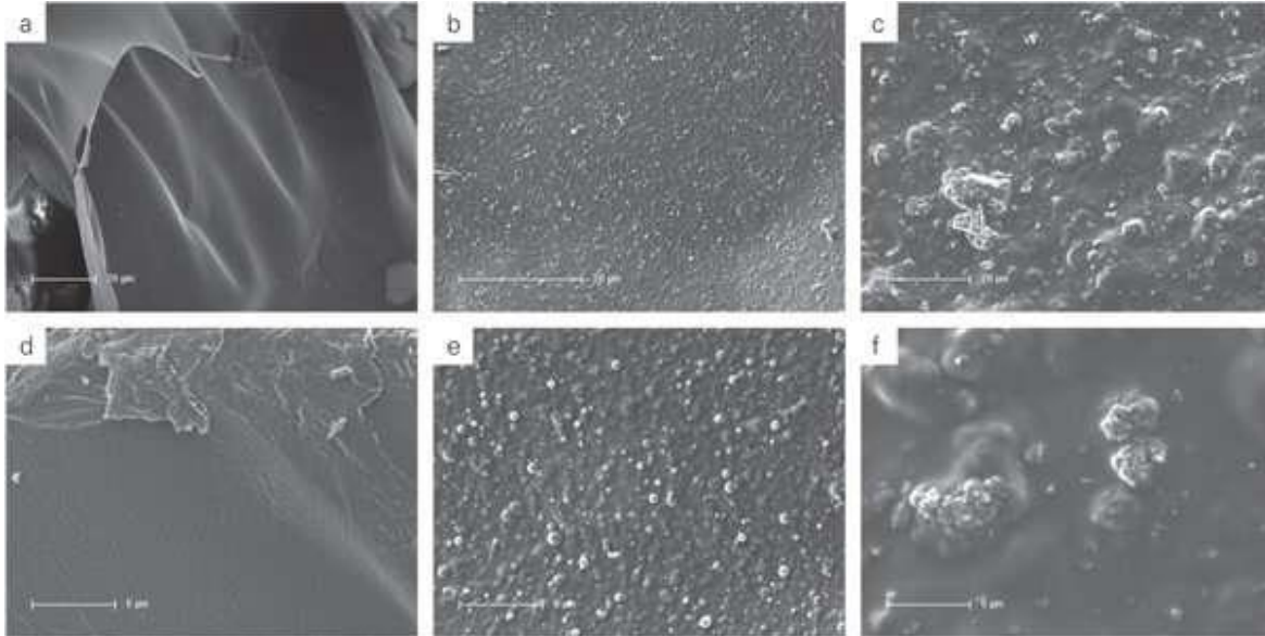
SEM images of foamed scaffolds without mineral (a), (d), with 20% ormoHAP (b), (e) or with 20% commercially available HAP (c), (f). Scale bars represent 20 \mu\text{m} (top column), and 5 \mu\text{m} (bottom column). Credit: Biomedical Materials, doi: 10.1088/1748-605X/ab0fad
