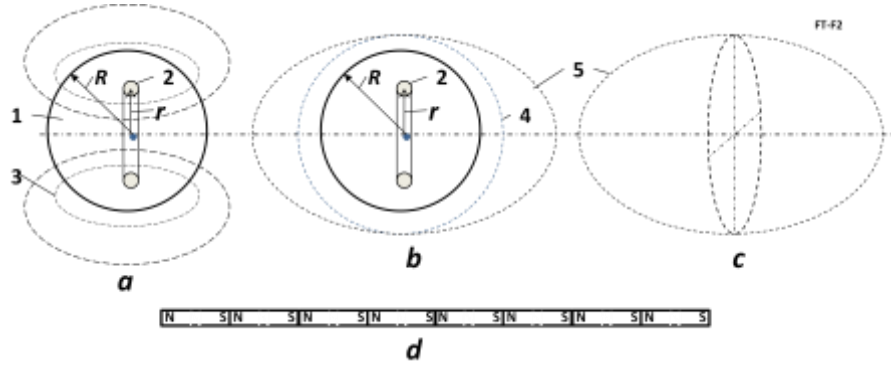
Fig.7. For computation of the magnetic force from the magnetic momentum of a nucleon (proton or neutron). Notations: a – nucleon: 1 – nucleon having radius R , 2 – electric current ring having radius r , 3 – magnetic lines from the magnetic momentum. b – magnitudes of forces near nucleon: 4 – nuclear and electrostatic forces, 5 – magnetic force. Magnitudes equal a distance from the center to the dot line. c – form of forces in isometric view. Form is closed to a rotated oval or rotated ellipsoid. d – is AB needle from nucleons connected in line as magnets.
