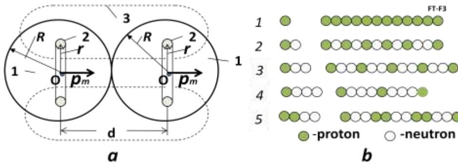
Fig.8. Left: Two connected nuclei work as solenoid. Their magnetic force is increased. 3 is common magnetic lines. Right: AB-needles: Notations: 1 – AB-needle from protons (pppp...); 2 – AB-needle from one proton + one neutron (pnpn...); 3 – AB-needle from one proton + two neutrons (pnmnpn...); 4 – AB-needle from one proton + three neutrons (pnnnpnn...), 5 – AB-needle from two protons + two neutrons (ppnppnn...)(ends have one proton).
