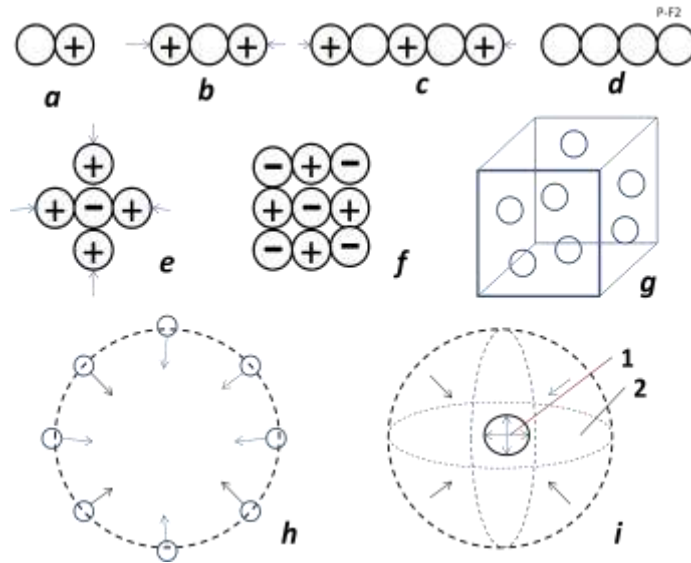
Fig.2. Constriction (structures) from eners. Notations: a) Neutral pairs of; b) Charged triple; c) Tread (rod) from eners ; d) Magnetic construction; e) Complex charged construction ; f) Plate charged construction; g) Volume construction; h) Circle construction; i) Spherical construction (1 – core, 2 – pressure cloud from eners).
