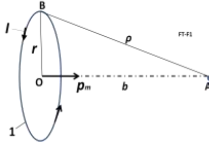
Fig.6. For theory of the magnetic intensity in an axis of the circle currency having the magnetic momentum p_m . Notations: A is point where we measure the magnetic intensity H ; 1 – current circle is creating the electric charge: r is radius, I is electric currency, p_m is magnetic momentum; b is distance of line OA; \rho is distance AB.
