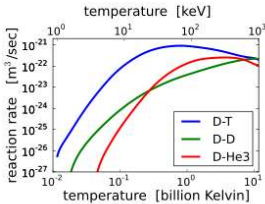
Fig.2. Reaction rate \langle \sigma v \rangle via plasma temperature for D-T (top), D-D (middle) and D- ^3\text{He} (bottom in left side).
