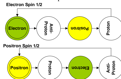
FIGURE 3. Dimensional notes associated with Electron and Positron. Lighter = positive charge, darker = Negative charge, White = Invisible in 3D due to 4D orientation – perpendicular to the Fabric of Space.
