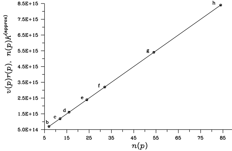
Figure 4: Comparison of real data v(p)r(p) ( \times ) with the formula n(p)K^{(approx)} ( \circ ) for the system HD10180.
