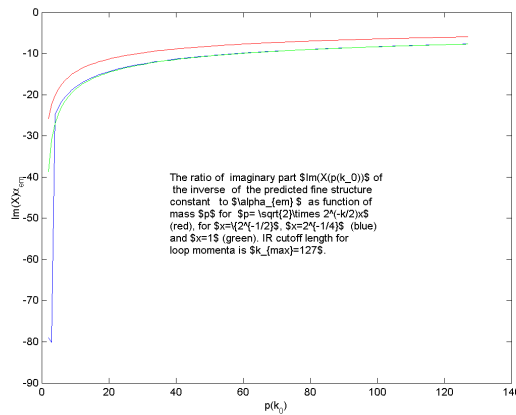
Figure 10.1: The evolution of the ratio r = \alpha_{em}/\alpha_{em,pred}(p) , where \alpha_{em} is the experimentally determined value of the fine structure constant at electron length scale and \alpha_{em,pred}(p_k) for p_k = \sqrt{2}m_k = 2^{-(k-1)/2}xm(CP_2) , k = 2, \dots, 127 , x \in \{2^{-1/2}, 2^{-1/4}, 1\} . Note that the three points correspond to the lower end, middle point, and upper end of the p-adic mass scale range labeled by the integer k_0 .
