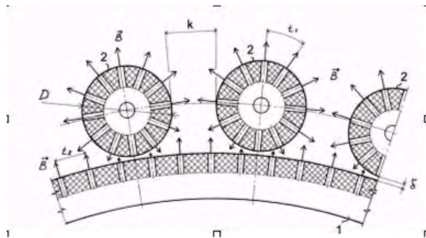
Figure 4.1: Variant of one-ring converter (figure 25 in [H36]).
